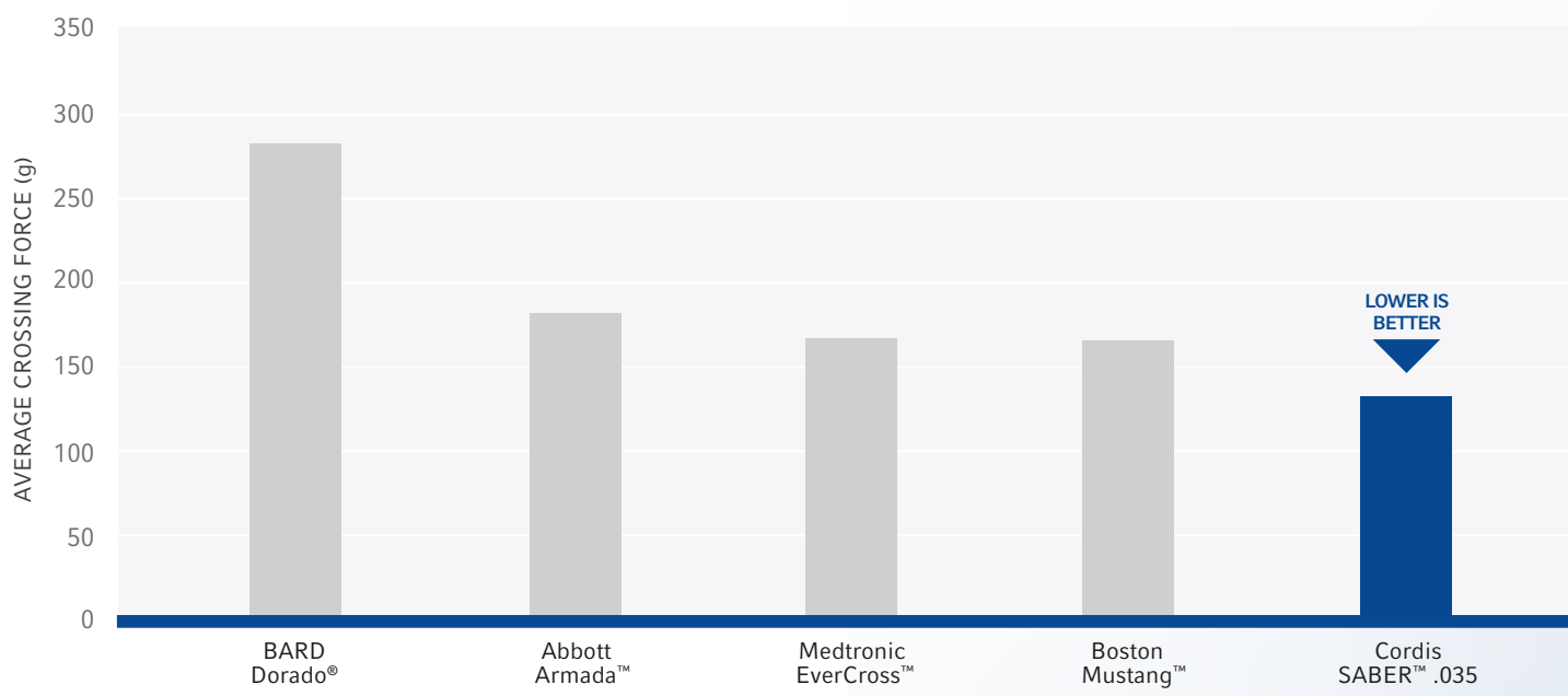
6 x 200 mm Superficial Femoral Artery (SFA) Crossing Model
